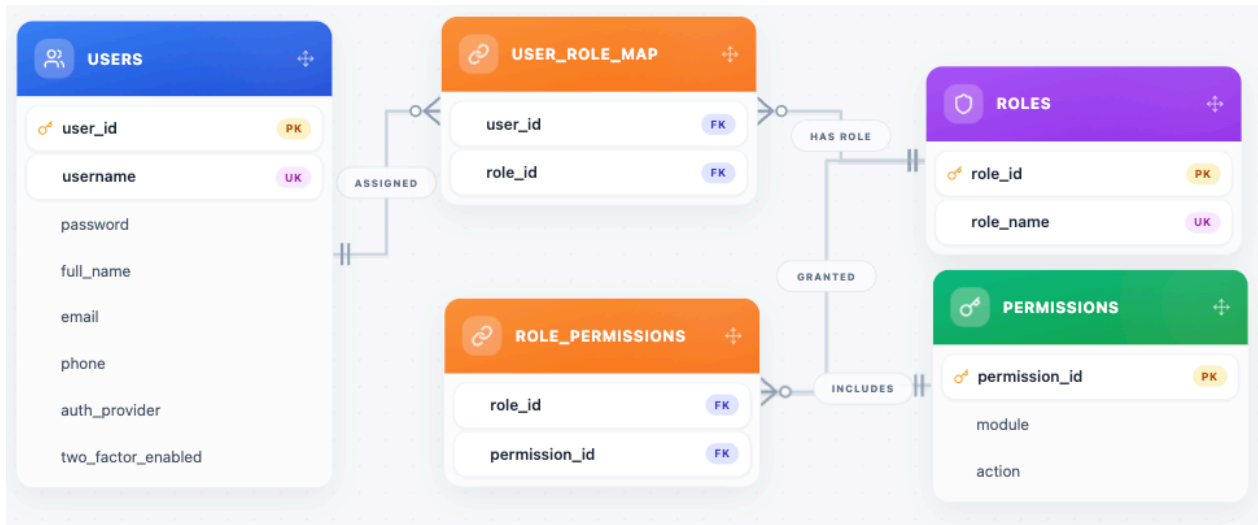
Figure 4-4: ER Diagram — User & Authentication Entities
