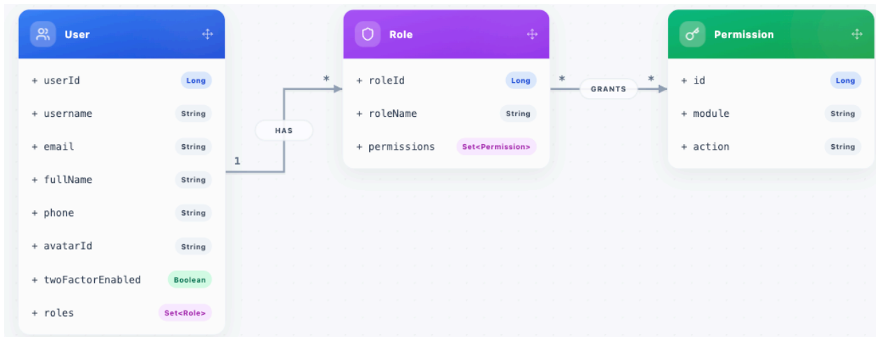
Figure 4-7: Class Diagram — Core User &amp; Authentication
