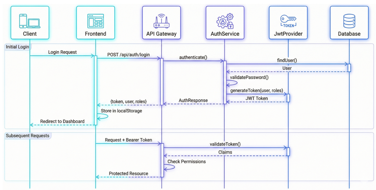
Figure 4-3: Main System Authentication and Request Flow
