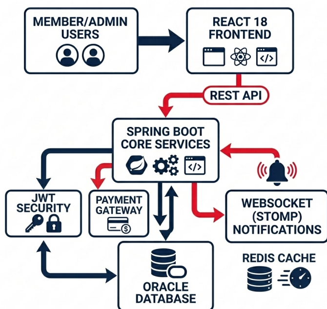
Figure 1: Full-Stack IT Architecture & Core Services
