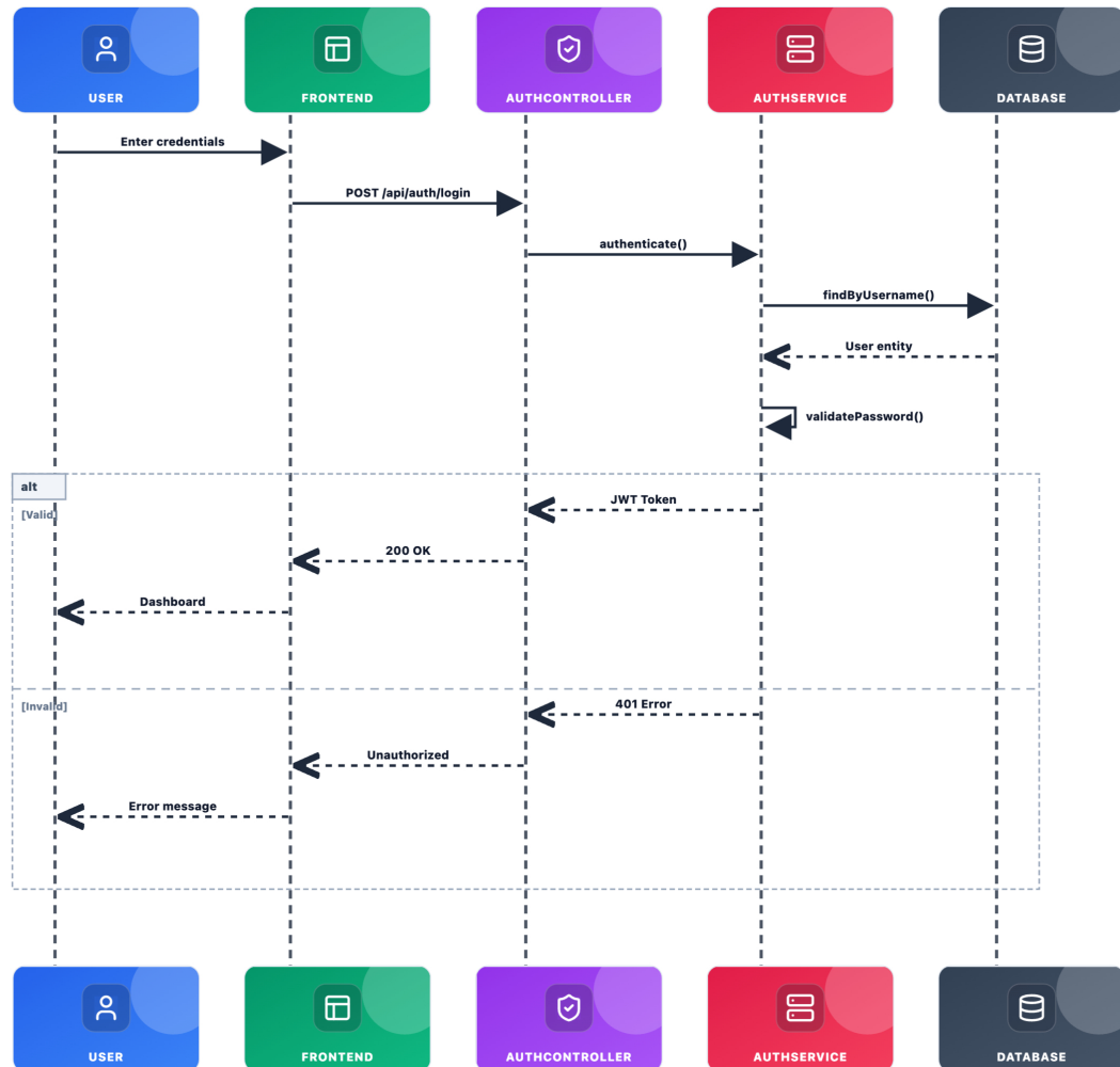
Figure 4-9: Sequence Diagram — User Authentication Flow
