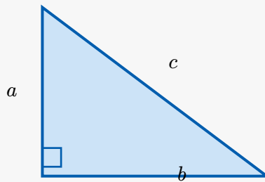
Figure 1: The standard configuration of a right triangle showing the orthogonal legs and the hypotenuse.
