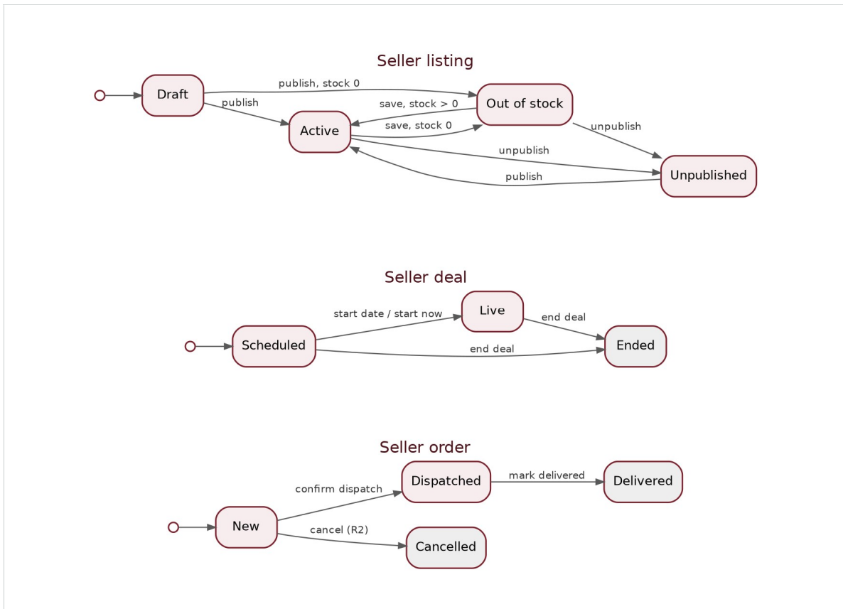
Figure 37: State diagrams: seller listing, seller deal, seller order
