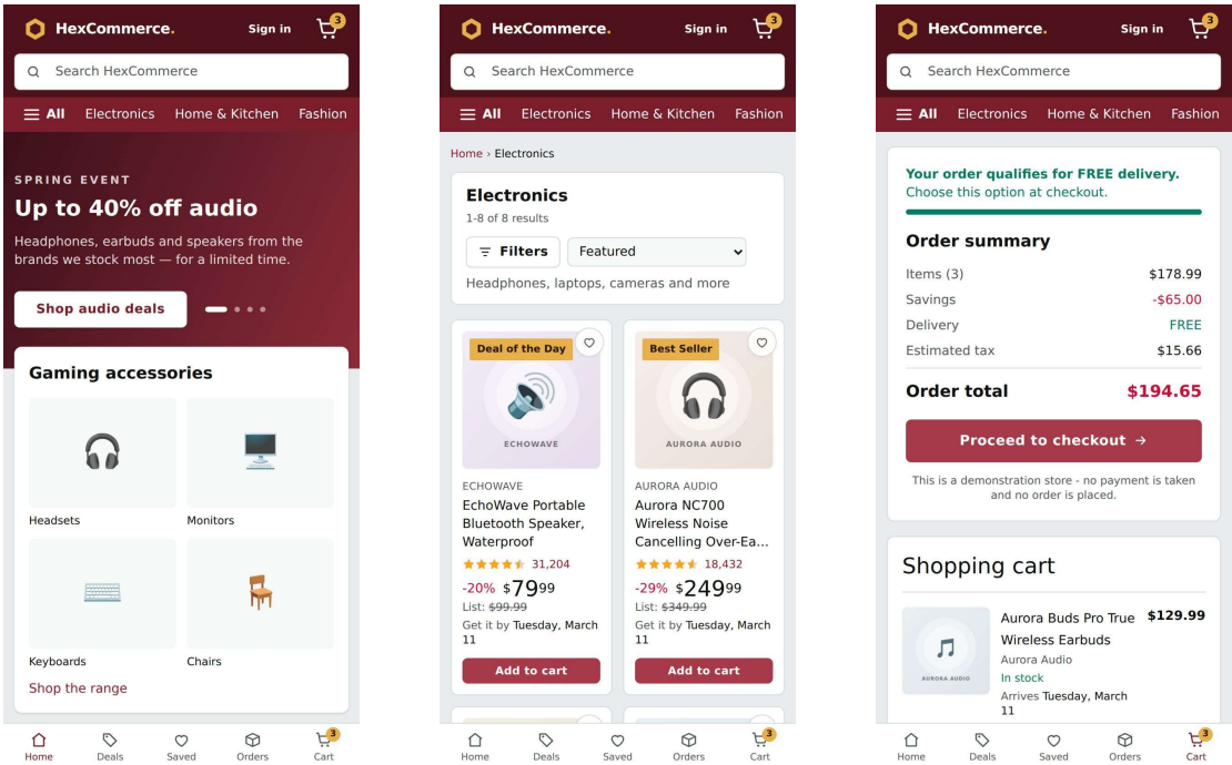
Figure 2: Phone layouts: home, department listing with Filters button, and basket with bottom tab bar
