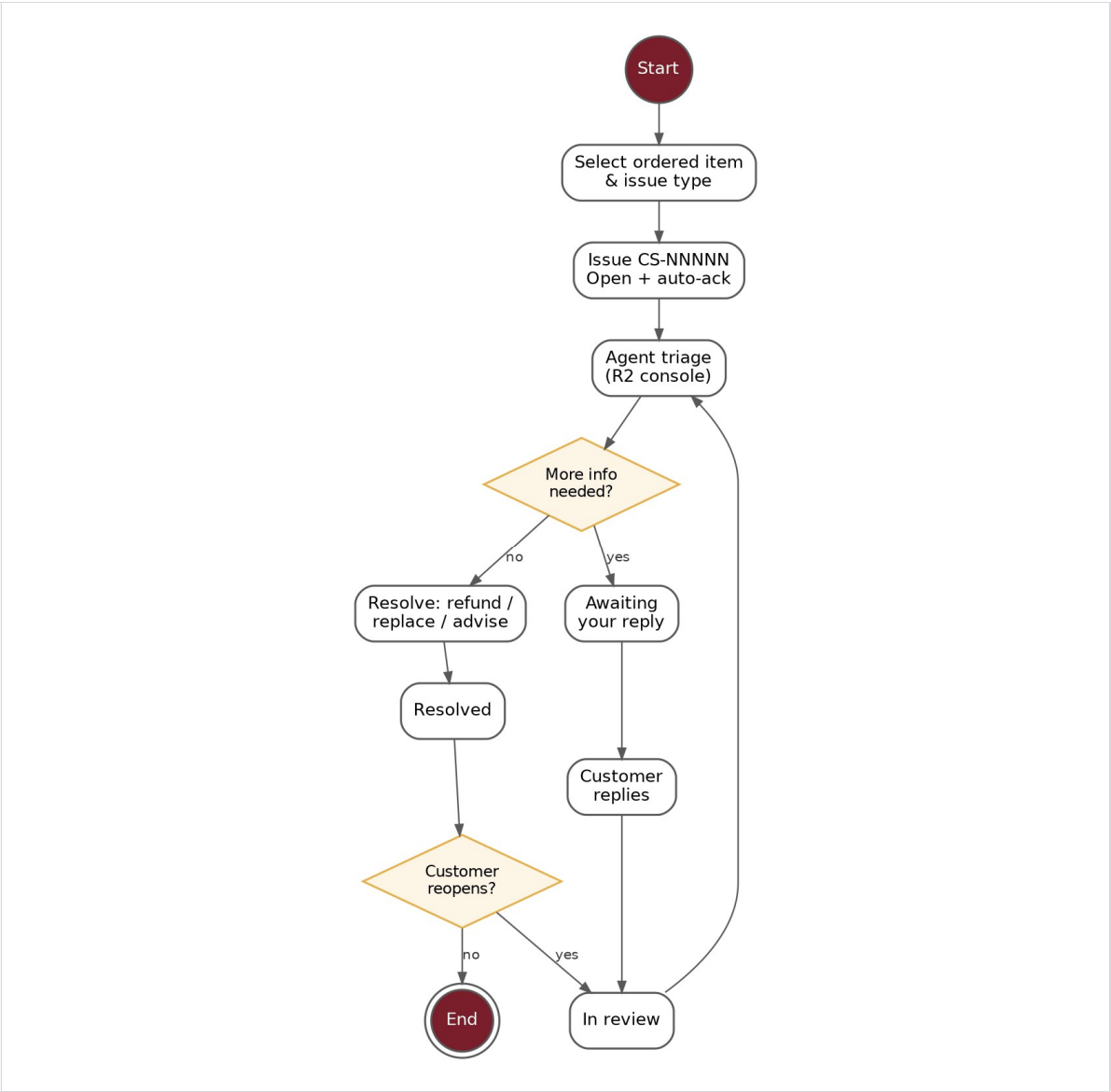
Figure 4: Process flow: support issue handling
