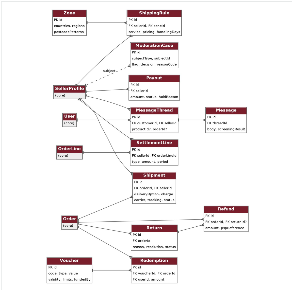
Figure 35: Logical data model – R2 entities and their links to core entities (grey)
