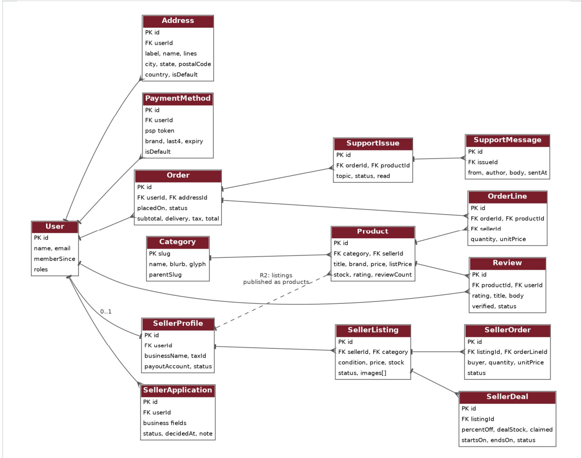
Figure 34: Logical data model – core entities
