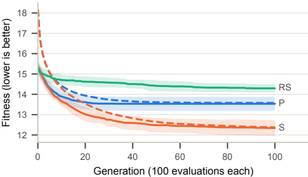
(a) Fitness
