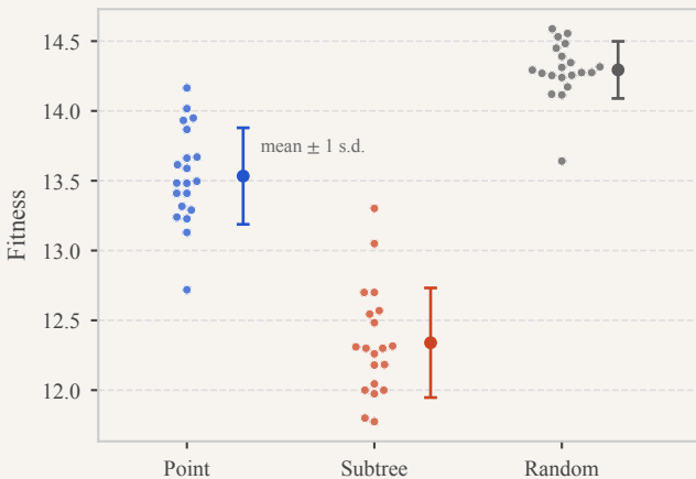
Final best fitness per run
