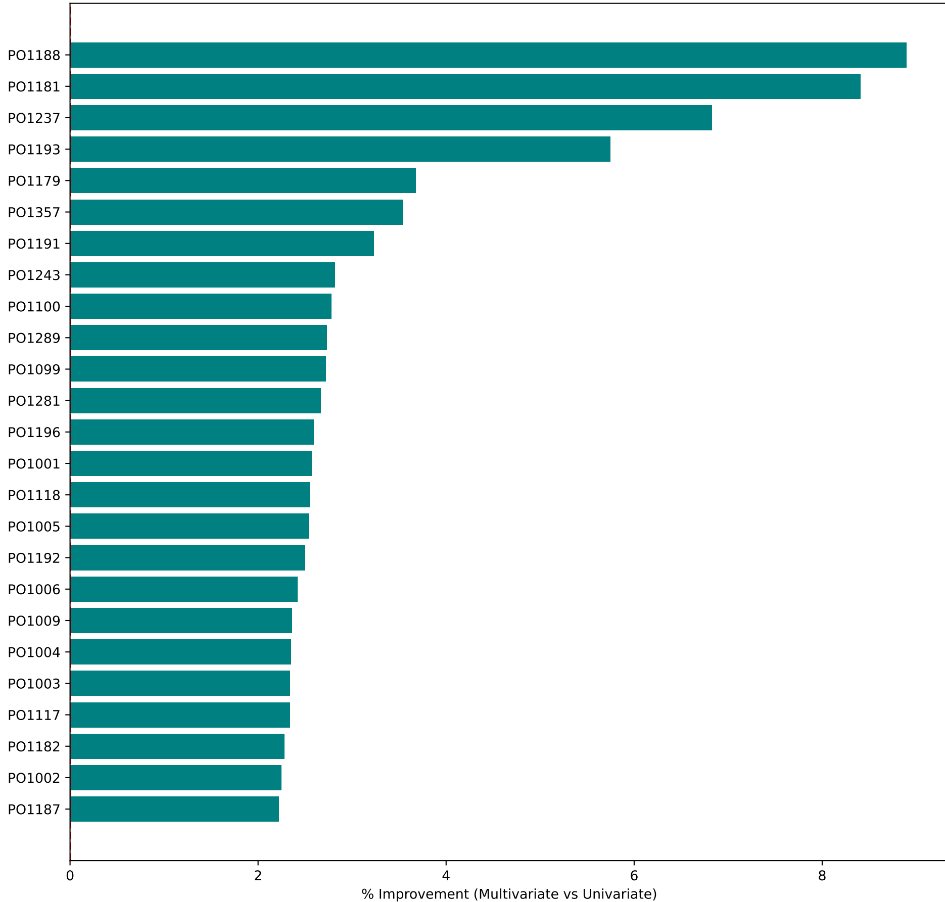
Experiment 2: Impact of Macroeconomic & Weather Features (Top 25 Products)
