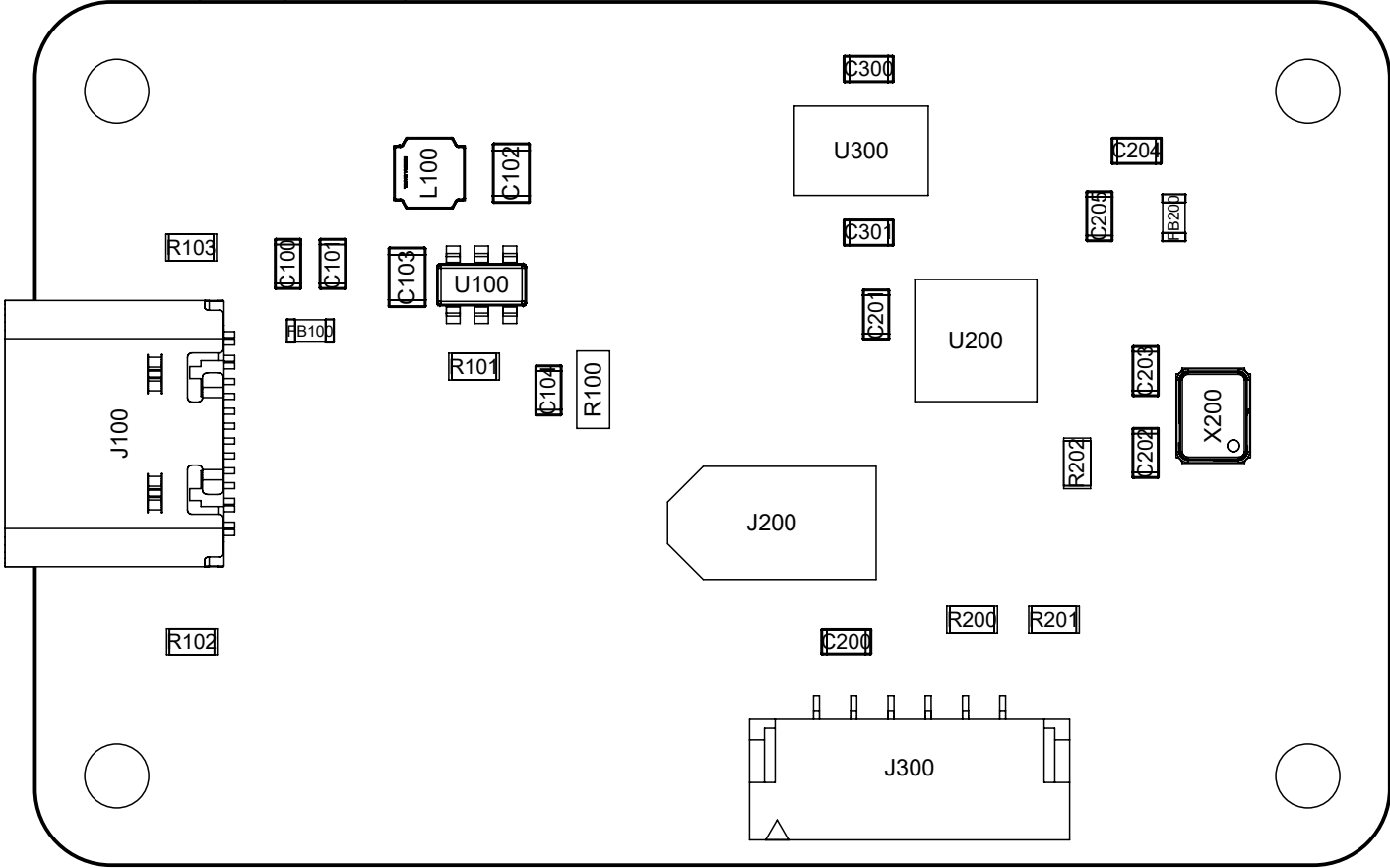
View from Top side (Scale 4:1)
