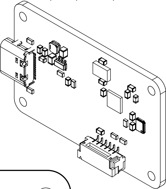
View from Top side (Scale 2:1)
