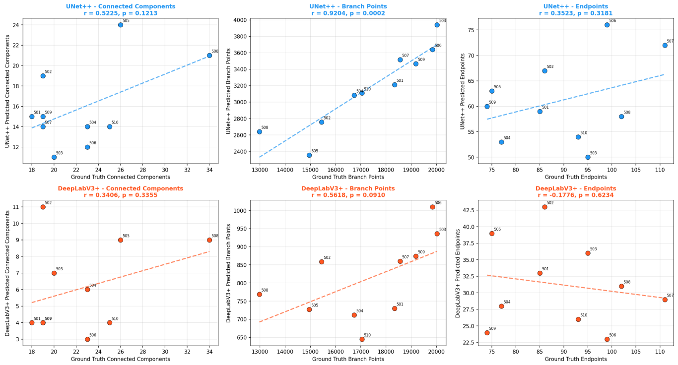
Pearson Correlation: Ground Truth vs Predicted Skeleton Properties (Each point = one test image)
