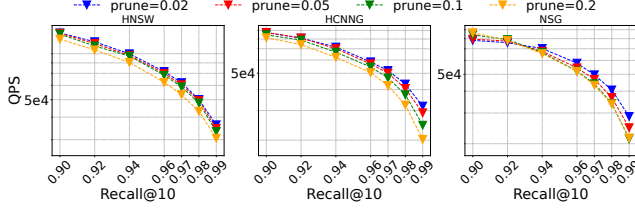
Figure 10: Impact of pruning ratio \rho on PIGR performance (QPS–Recall@10).
