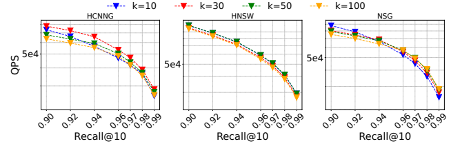
Figure 12: Impact of k size on PIGR performance (QPS–Recall@10).
