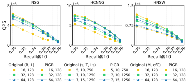
Figure 8: Effect of PIGR across multiple initial parameter configurations on DBPEDIA1M (QPS–Recall@10).
