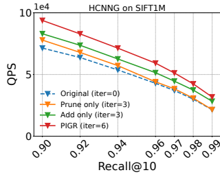
Figure 13: Independent effects of pruning and bridging on HCNNG with SIFT1M (QPS–Recall@10) under a matched refinement budget.
