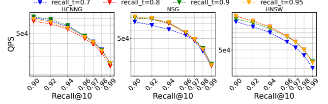
Figure 11: Impact of recall_{target} on PIGR performance (QPS–Recall@10).
