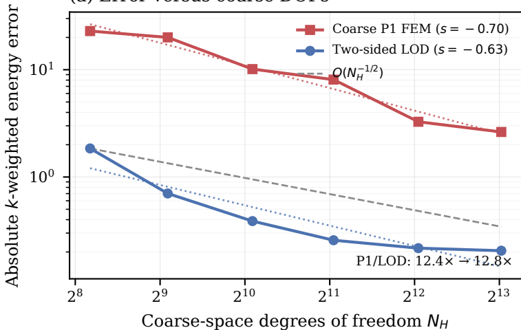
(a) Error versus coarse DOFs
