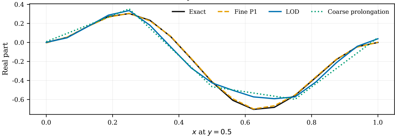
Fixed cross-section resolves the oscillatory correction
