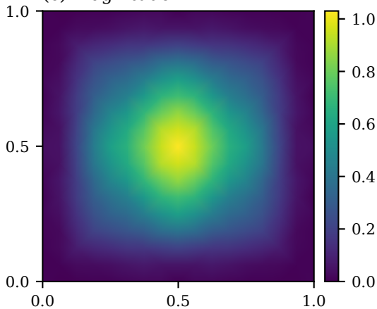
(c) Magnitude
