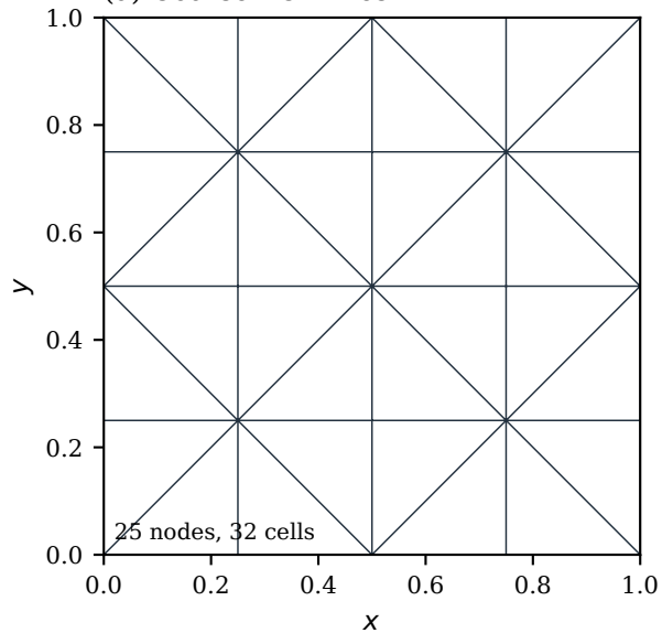
(a) Coarse LOD mesh
