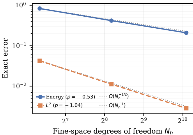
(a) Global-NVB fine P1 FEM
