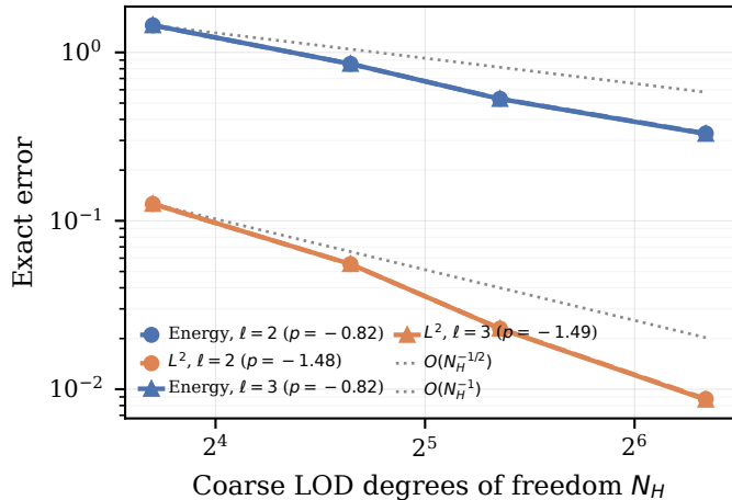
(b) Two-sided LOD, fixed fine level h = 10
