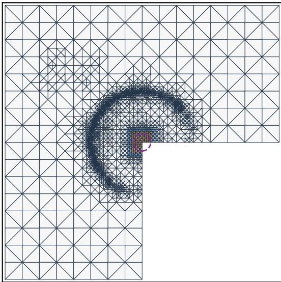
Final solved hybrid mesh
