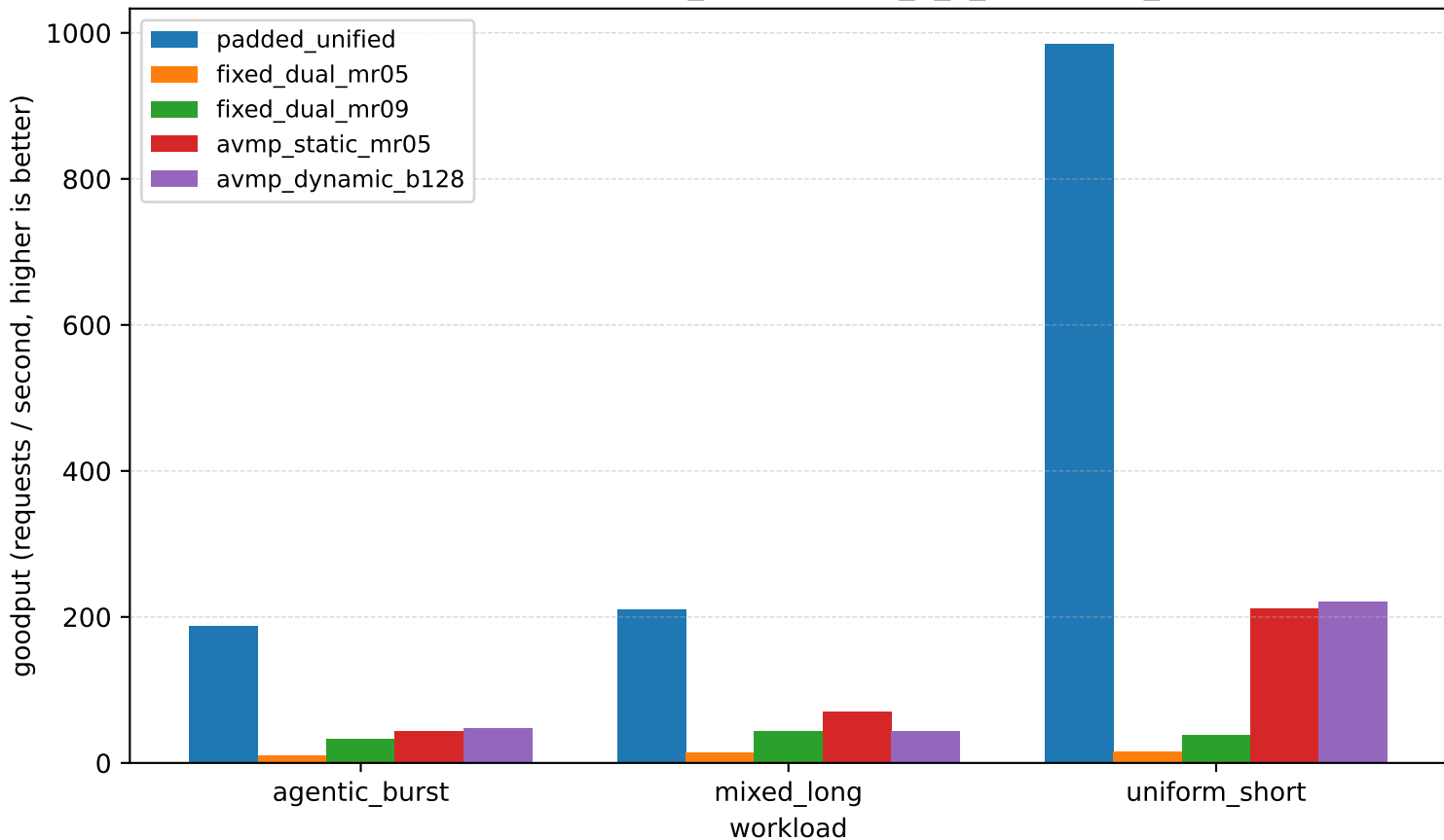
Goodput by workload (model_spec=jamba_1_5_mini, total_bytes=4gib)
