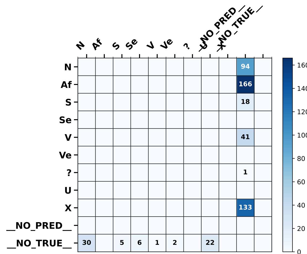
Predicted label
