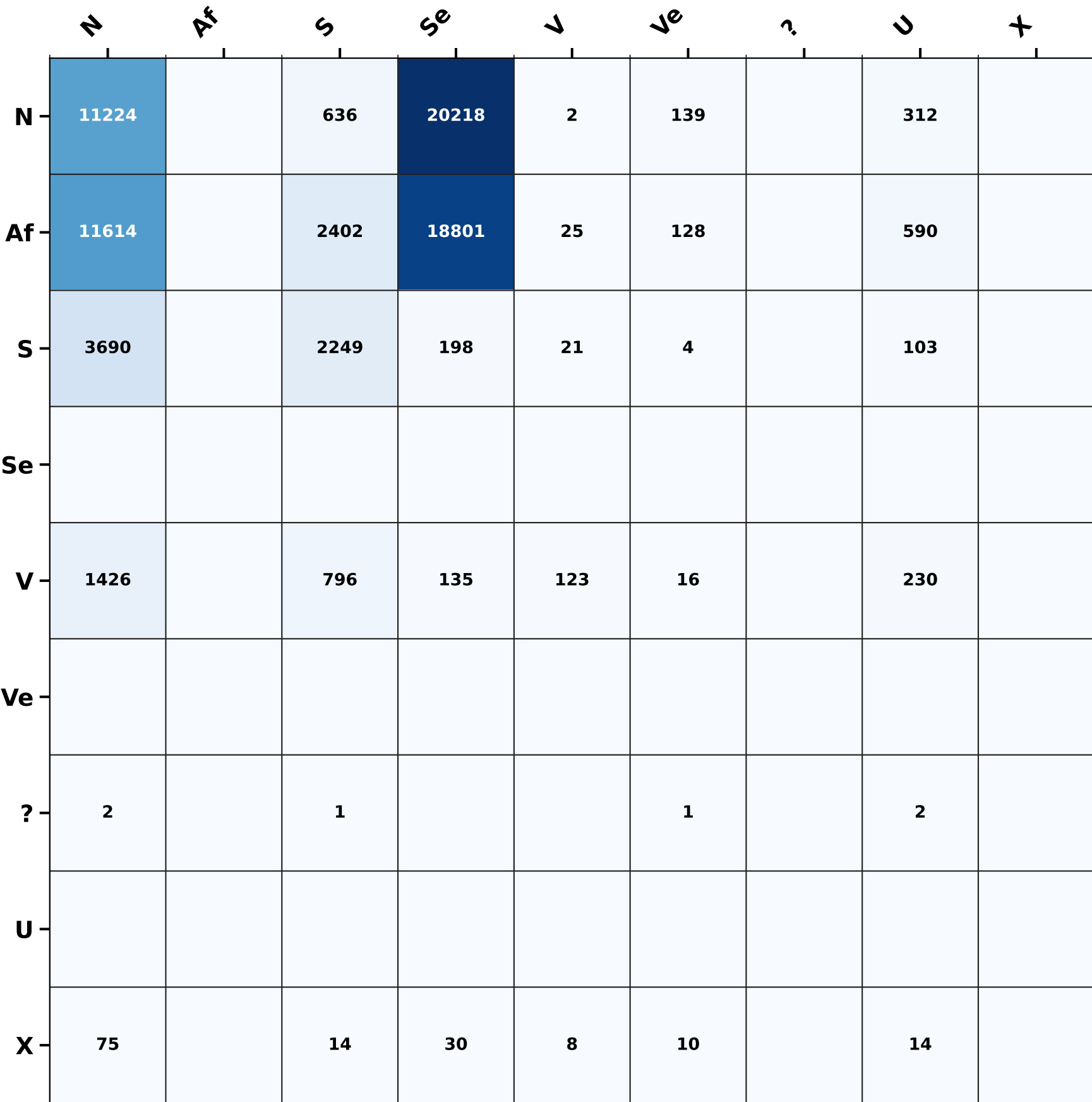
Predicted label
