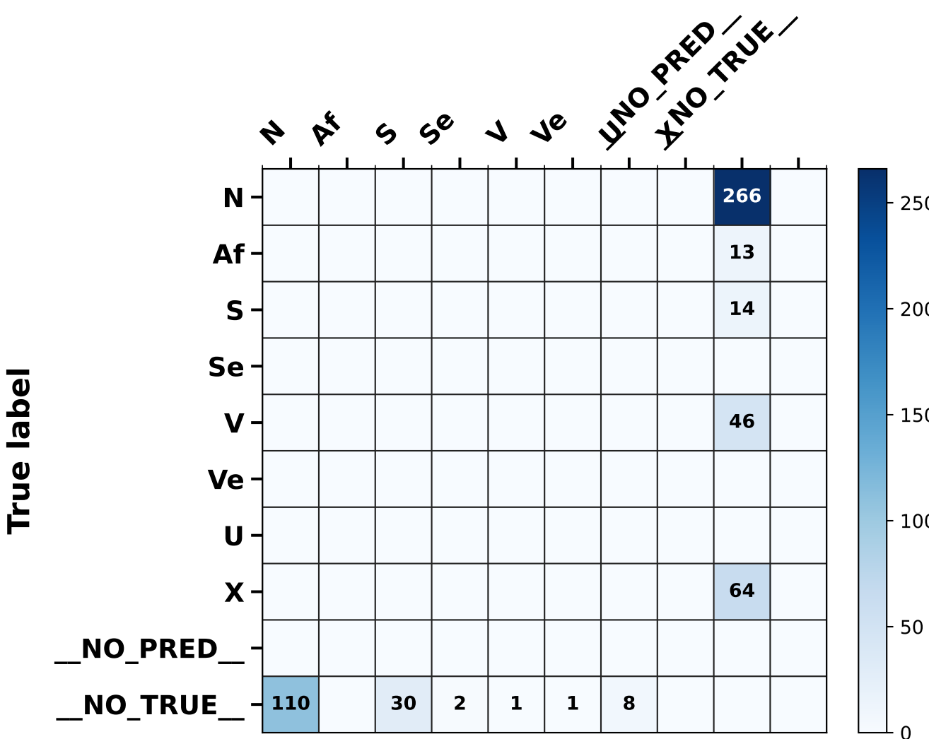
Predicted label
