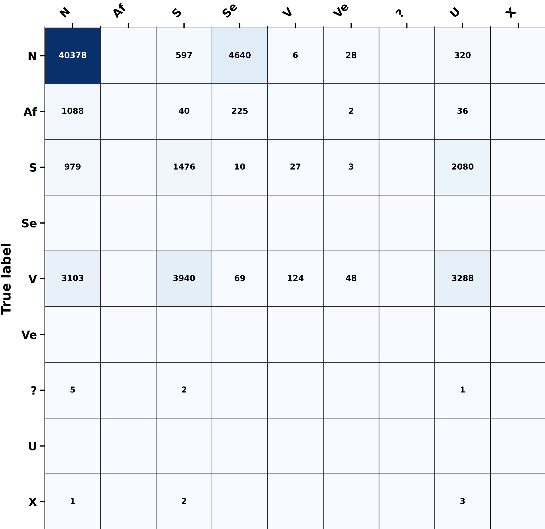
Predicted label
