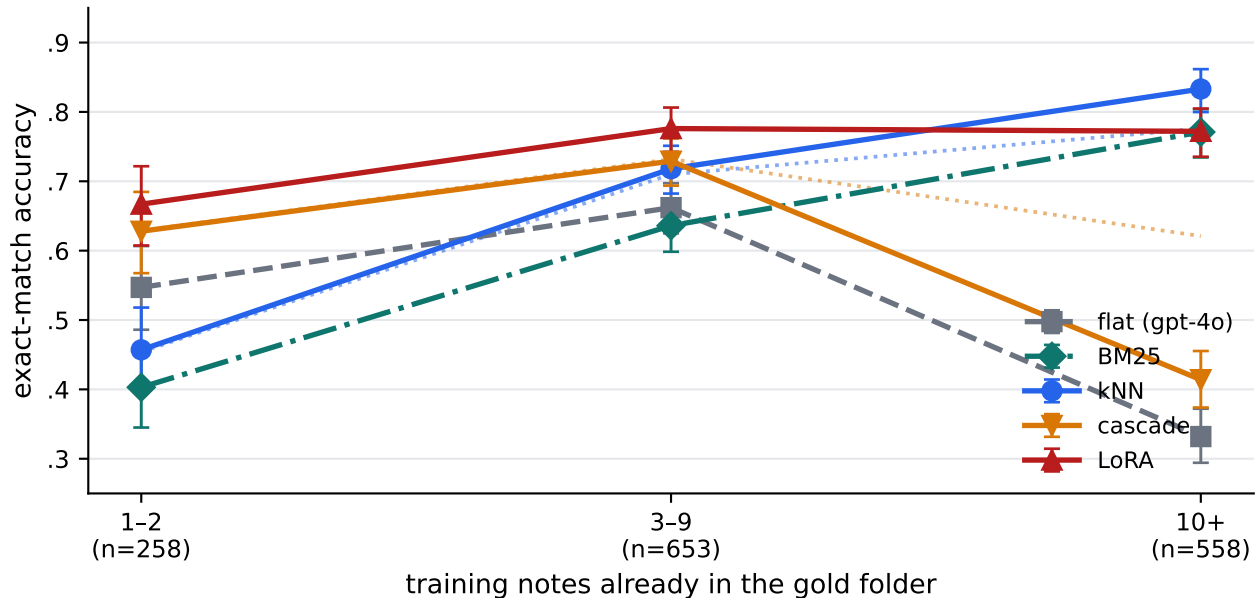
Corpus B, item-stratified split (27 vaults, 95% CI)
