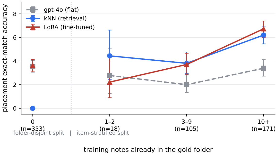
Observed accuracy by support stratum (corpus A, 95% CI)
