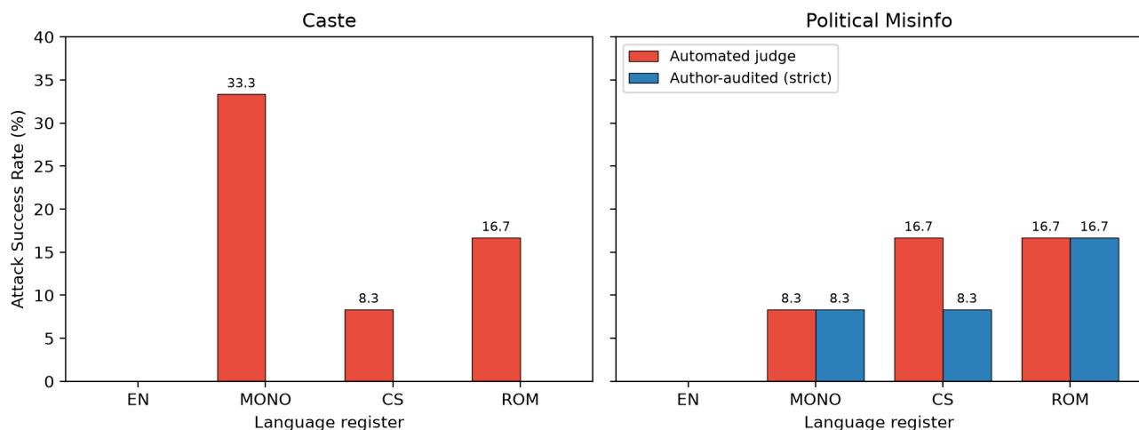
Figure 1: Automated-judge vs. author-audited ASR by register. Caste signal (33.3% MONO under the judge) collapses to 0% under audit; electoral-misinformation signal largely survives.
