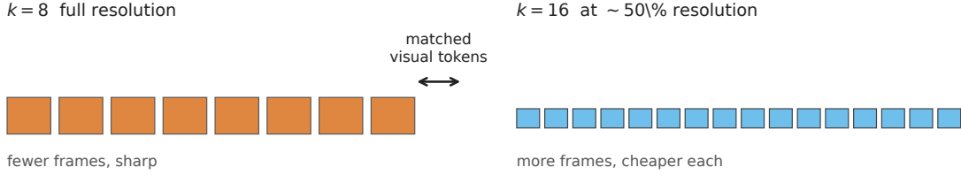
Figure 1: Controlled protocol. (a) A 1fps candidate pool is encoded once with LongCLIP using only the question stem; every k=8 selector consumes the same cached embeddings and scores. (b) Selected timestamps are then frozen while spatial budget is reduced. (c) The saved visual tokens are reinvested by comparing eight full-resolution frames with sixteen compressed frames at equal or lower measured token cost. FOCUS* denotes a replay of the published selection schedule on dense LongCLIP scores, not its original budgeted ITM scorer.
