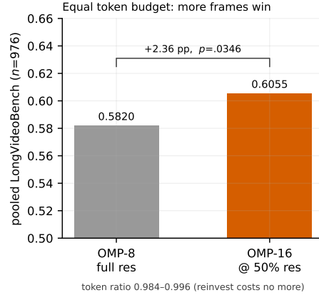
Figure 4: LongVideoBench 600 s and 3600 s pooled: sixteen compressed OMP frames outperform eight full-resolution OMP frames at a measured token ratio no greater than one.
