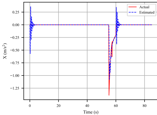
QUAV \#3
