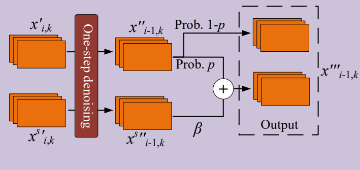
Stylized Latent Feature Fusion (SLFF)
