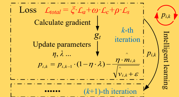
Learnable Intelligent Latent Perturbation (LILP)
