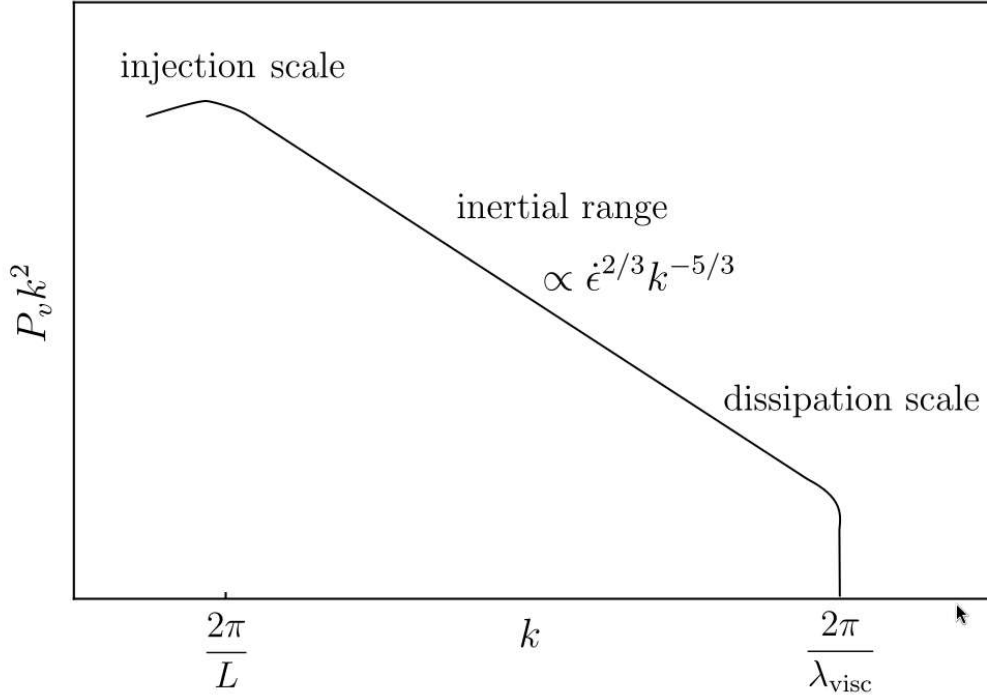
Figure 1.2: The three-dimensional velocity power spectrum P_v k^2 as a function of wavenumber k , illustrating the Kolmogorov turbulent energy cascade. Energy is injected at the driving scale 2\pi/L , transferred through the inertial range with the characteristic \propto \epsilon^{2/3} k^{-5/3} scaling, and dissipated at the viscous scale 2\pi/\lambda_{\text{visc}} . In the ICM context, the injection scale corresponds to the dominant energy driver — merger shocks, sloshing, or AGN activity — while the dissipation scale is set by the effective viscosity of the weakly collisional plasma. This is also angle averaged also known as the omnidirectional spectrum.
