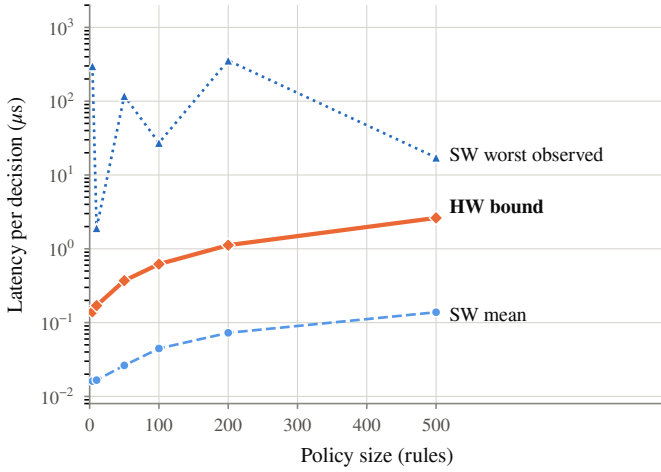
Fig. 3. Wall-clock latency per decision, log scale. The software mean and worst observed come from perf measurements of the five-dimensional path. The hardware line is the closed-form bound of (4) at 100 MHz, where minimum, mean and maximum coincide. The software worst case is an observation, not a bound, and does not track policy size.
