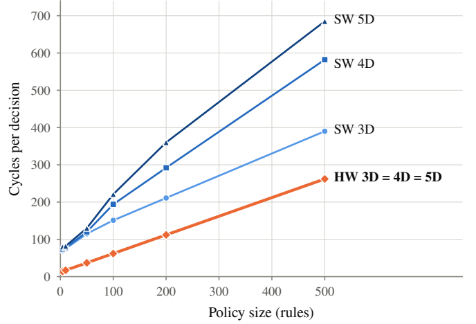
Fig. 2. Cycles per decision versus policy size. Software cycles are derived from perf-measured means and the 4.96 GHz clock; hardware cycles are co-simulated. Software slopes steepen with each added dimension. The 3D, 4D and 5D hardware series are identical at every measured point and render as one line.
