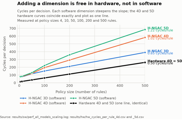
Fig. 1. Cycles per decision versus policy size. Software slopes steepen with each added dimension. The 4D and 5D hardware series are identical at every measured point.
