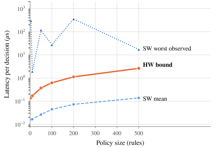
Fig. 2. Wall-clock latency per decision, log scale. The software mean and worst observed come from perf measurements of the five-dimensional path. The hardware line is the closed-form bound of (4) at 100 MHz, where minimum, mean and maximum coincide. The software worst case is an observation, not a bound, and does not track policy size.
