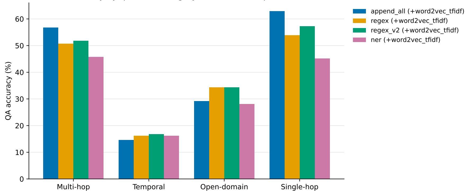
QA accuracy by question category (best retriever per extractor)
