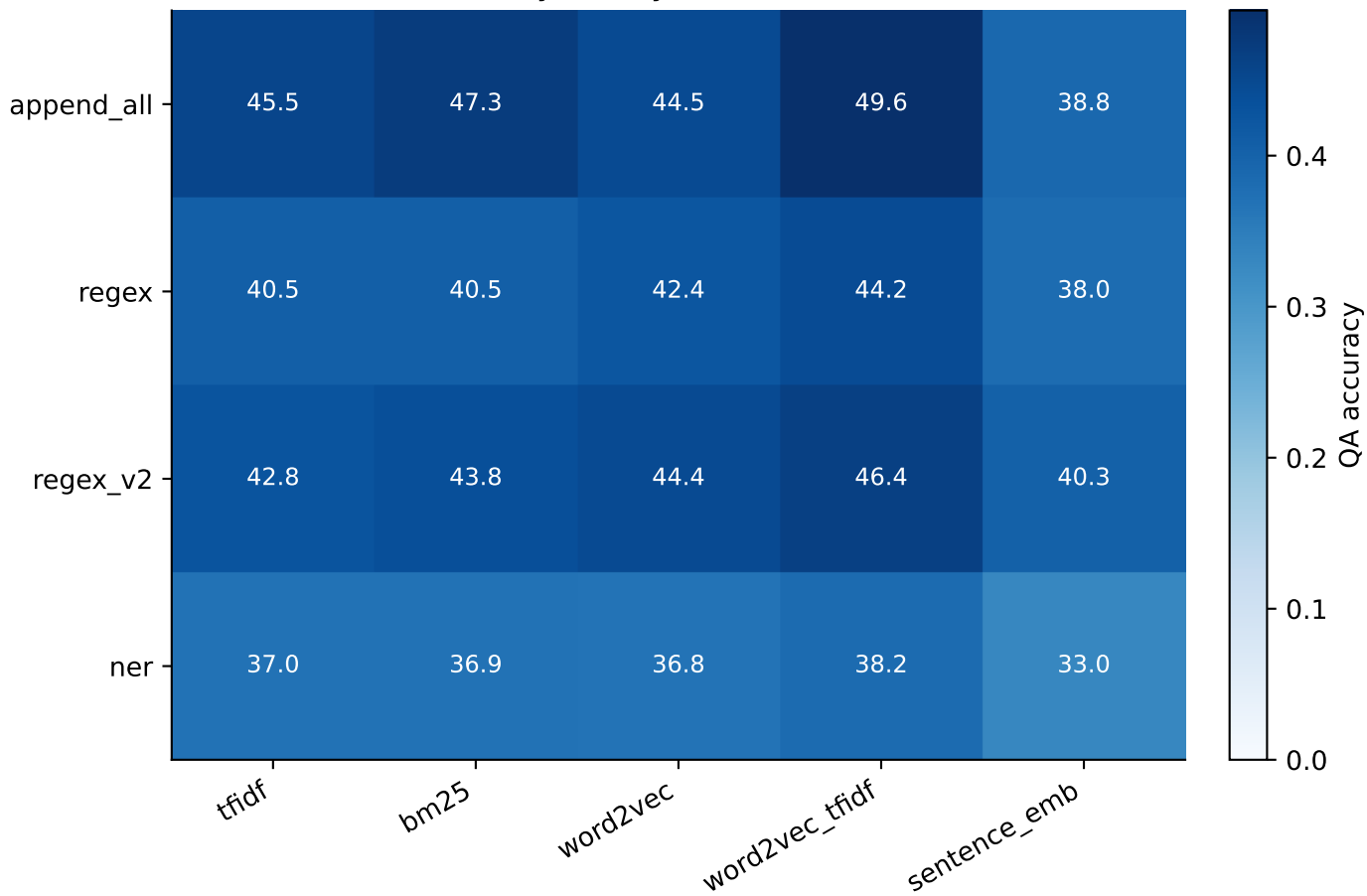
QA accuracy (%) by extractor x retriever
