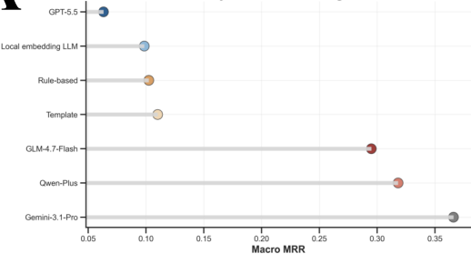
Modality-section retrieval alignment
