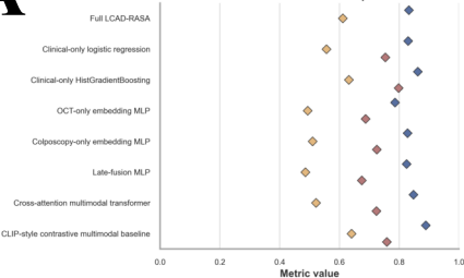
External baseline metric profile
