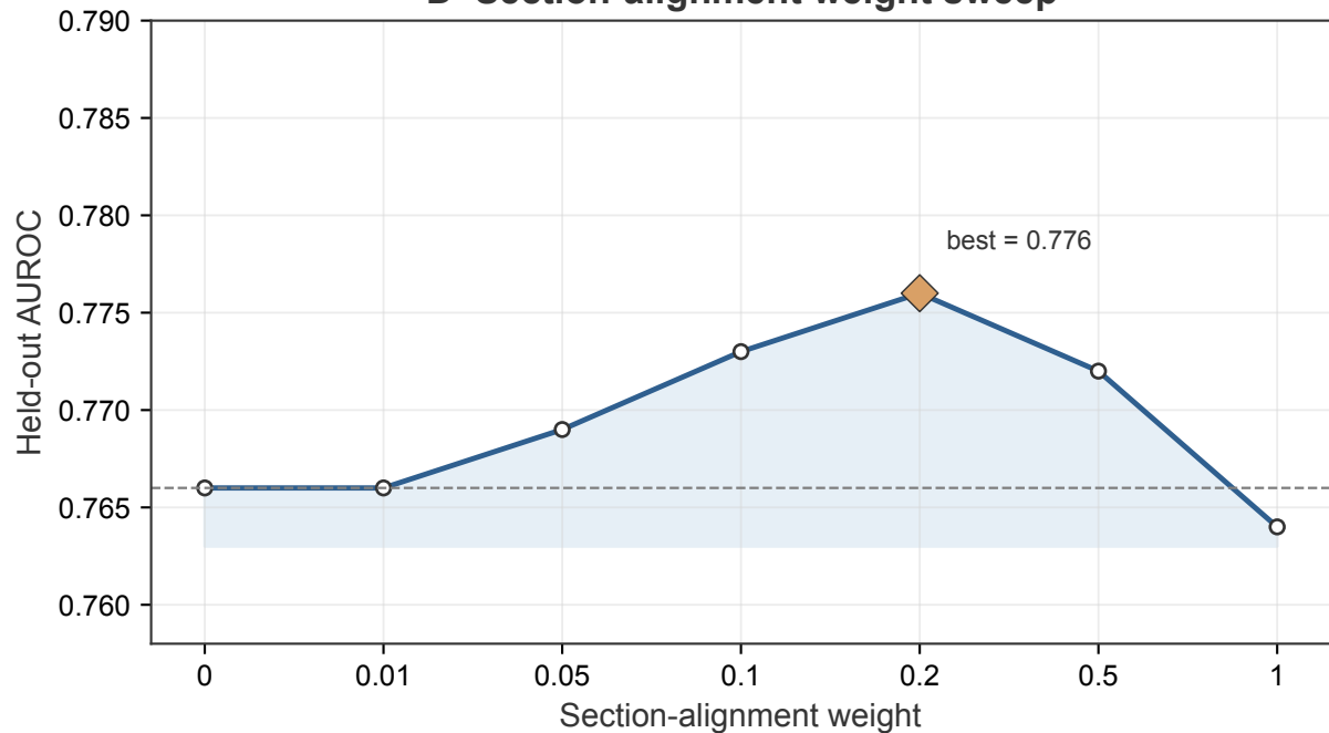
D Section-alignment weight sweep
