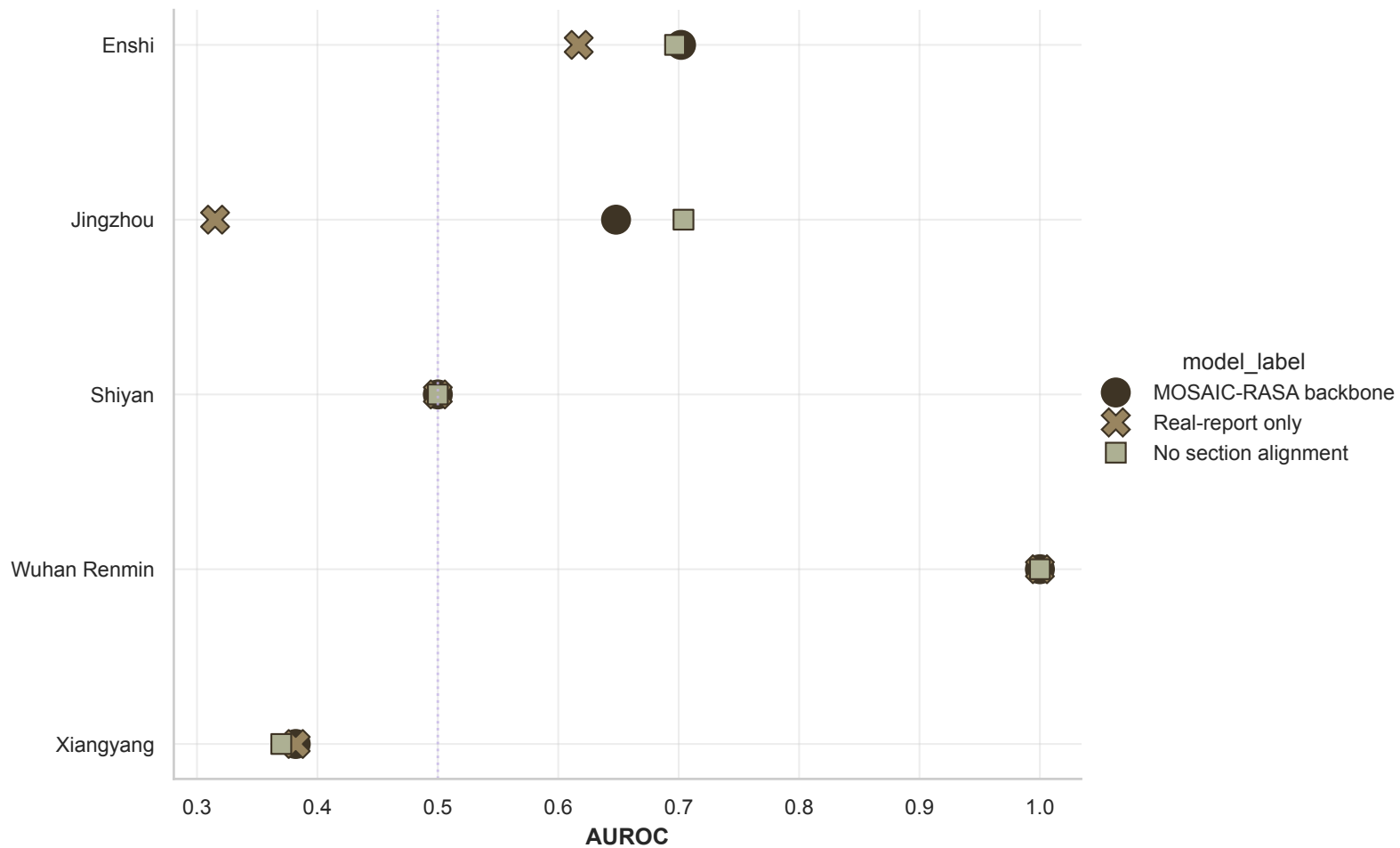
Strict LOCO AUROC by centre and model
