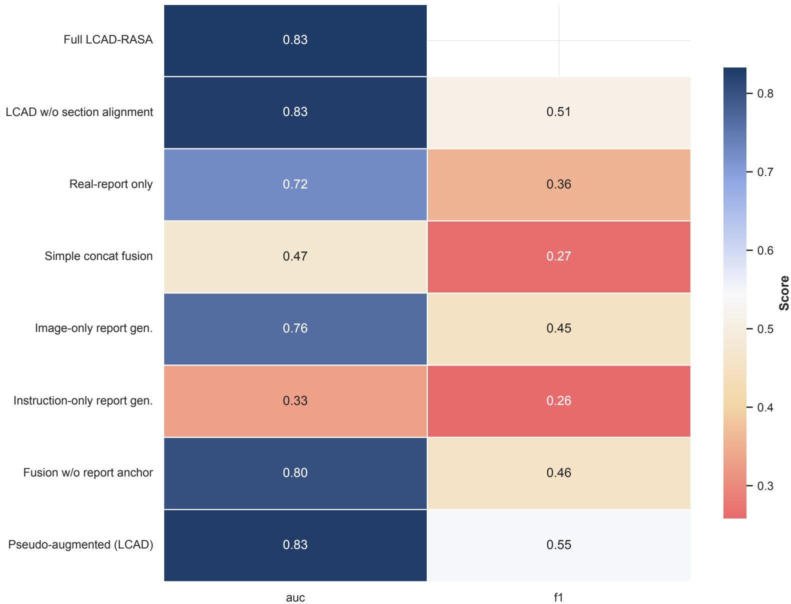
Multi-metric held-out performance profile
