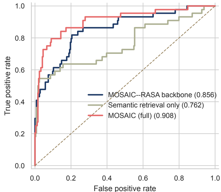
MOSAIC improves held-out risk stratification (delta AUROC 0.053, 95% CI 0.012 to 0.101, p=0.005 )
