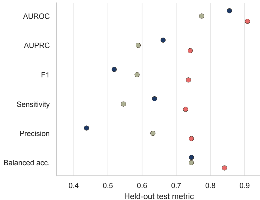
MOSAIC improves held-out risk stratification (delta AUROC 0.053, 95% CI 0.012 to 0.101, p=0.005 )
