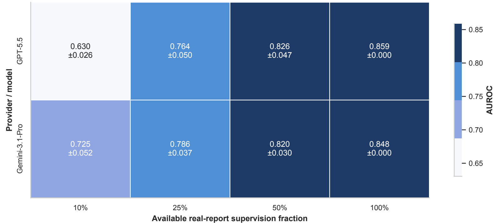
Downstream performance under report-supervision scarcity
