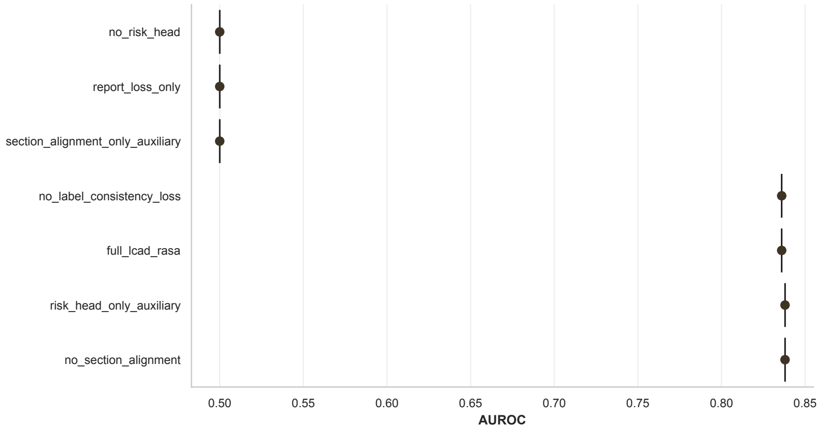
Rasa Component Boxenplot
