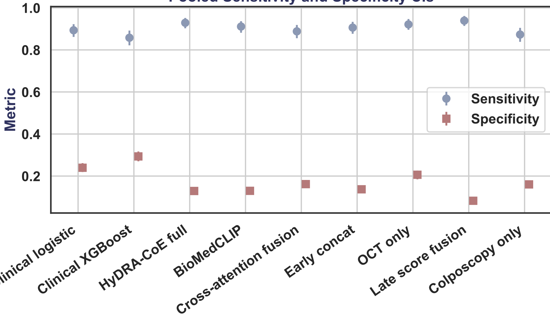
Pooled Sensitivity and Specificity CIs
