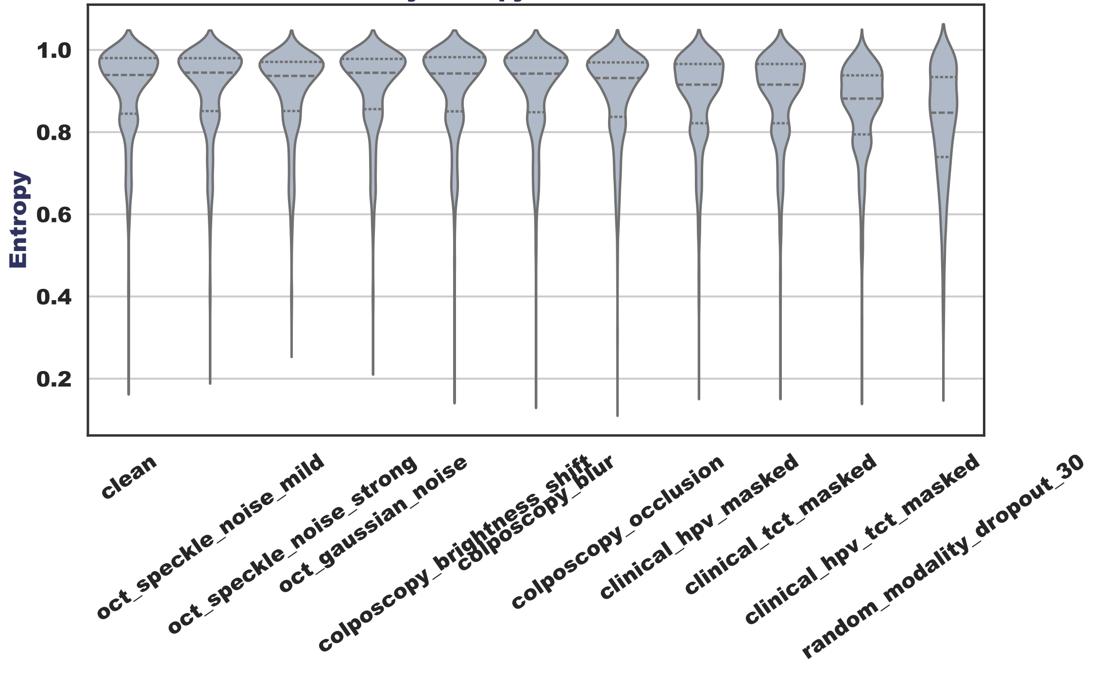
Reliability Entropy Under Perturbation
