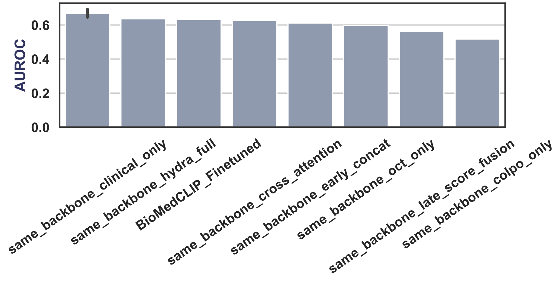
Available Same-Backbone/Fusion Control AUROC
