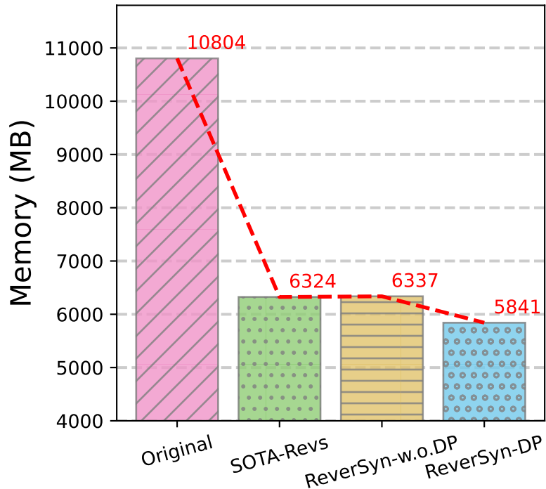
ResNet101
