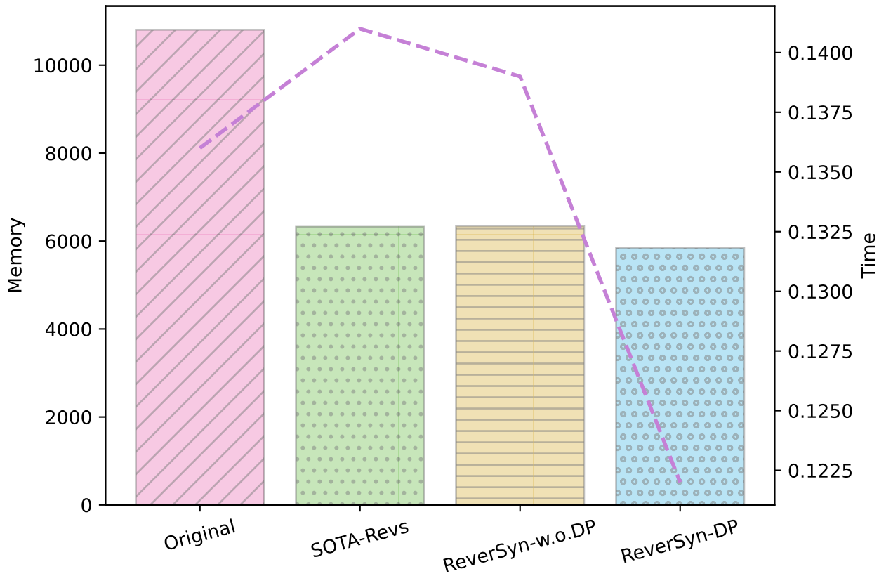
ResNet164
