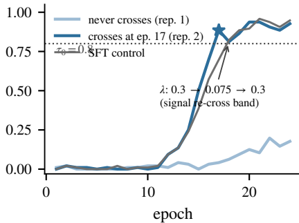
(b) 1.7B, output gate ( \rho = A_{\text{mem}}^{\text{lf}} )
