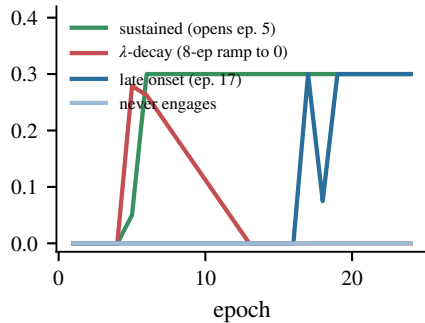
(c) engagement schedules \lambda(t) , 1.7B
