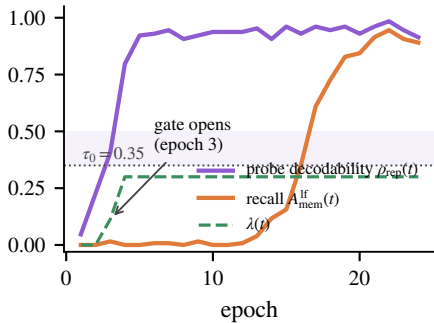
(a) 0.5B, probe-saturation gate
