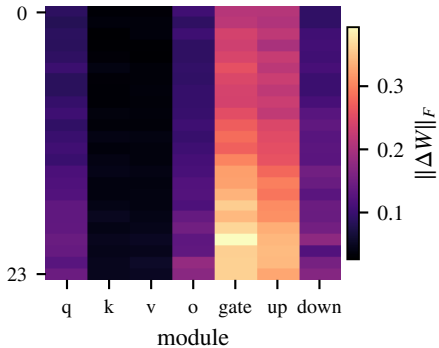
(a) 0.5B final adapter (layer \times module)
