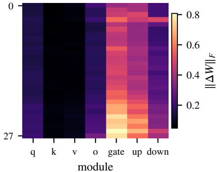
(b) 7B adapter (epoch 26)
