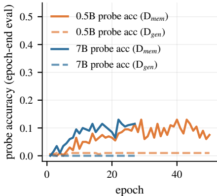
(a) Probe reads memorization ( D_{mem} \gg D_{gen} )
