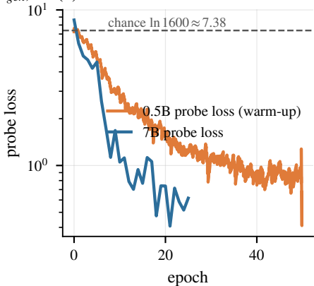
(b) Probe loss falls far below chance
