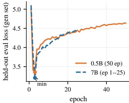
(b) Eval-loss reversal
